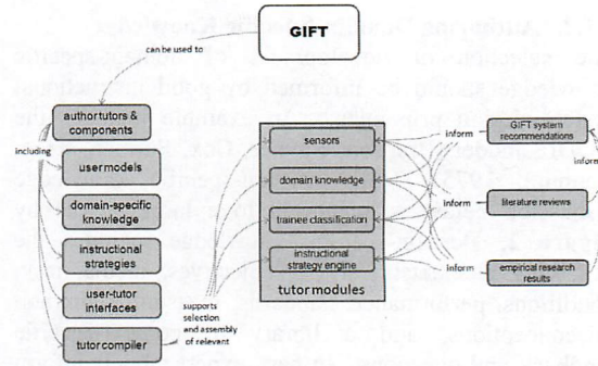
Figure 6: Tutor Compilation
