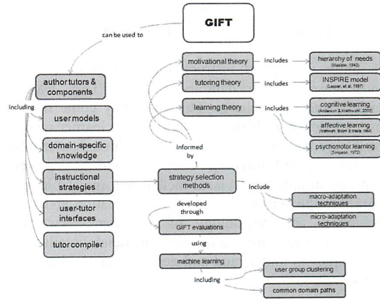
Figure 3: Authoring Instructional Strategies
