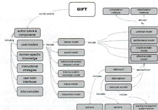
Figure 1: Authoring User Models
