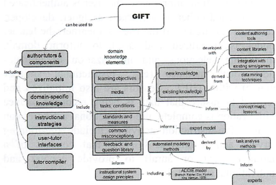
Figure 2: Authoring Domain-Specific Knowledge
