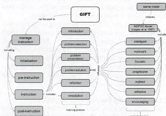
Figure 7: Tutoring Processes and Tutor Behaviors
